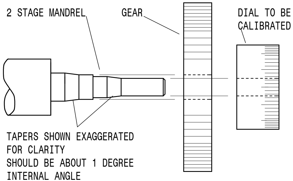
TWO STAGE TAPER STUB MANDREL SK. 5
