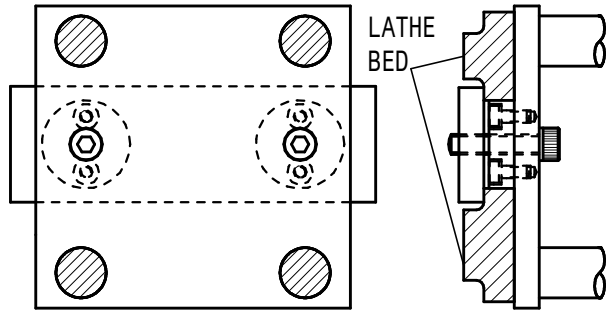
SUGGESTED MOUNTING FOR A SQUARE BED LATHE MOUNTING ASSEMBLY AS4
