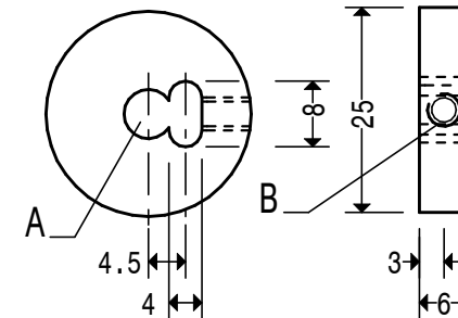
HOLES. A. 6 B. M4 MATERIAL 25 DIA. STEEL 230M07 QUANTITY 1 OFF SETTING PIECE 2
