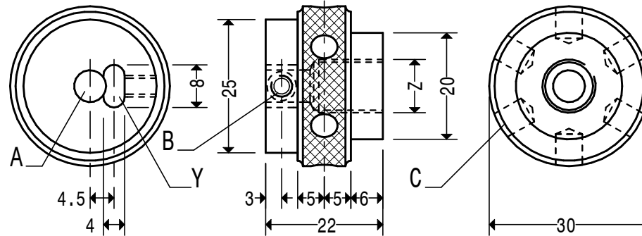
HOLES. A. 6 B. M4 C. 5.1 X 6 DEEP 6 OFF. Z. 3/8" X 32 TPI ME THREAD X 12 DEEP Y. MAKE RECESS 6 DEEP MATERIAL 30 DIA. STEEL 230M07 SECURING NUT 3
