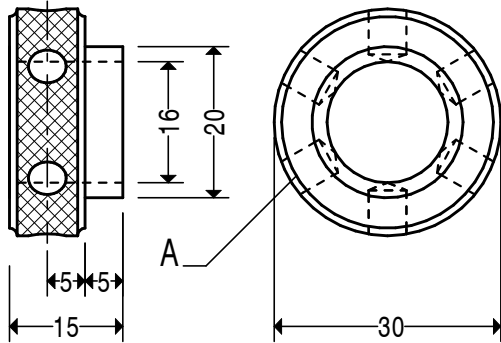
HOLES. A. 5.1 X 6 DEEP 6 OFF. MATERIAL 30 DIA. STEEL 230M07 QUANTITY 1 OFF HEAD 4
