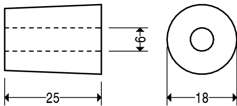
MATERIAL 20 DIA. STEEL 230M07 TAPER, AS NUMBER TWO MORSE QUANTITY 1 OFF STOP BAR SUPPORT 7
